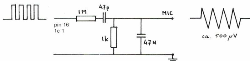
Fig. 3: Differentiator-integrator netwerk in ZX 81.
